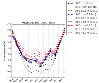
tempDC-FHLR9V60102_2000_2000
