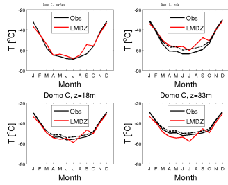
temp_DC_FHLR9V60102_2000_2000
