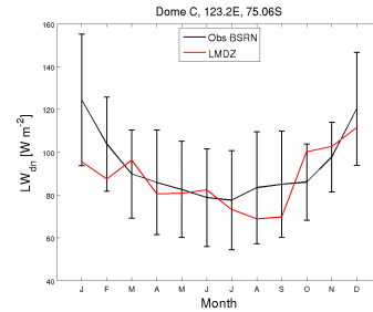
LWdnSFC_DC_FHLR9V60102con_2000_2000
