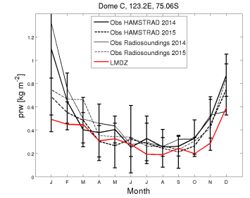
prw_DC_FHLR9V83_2000_2000
