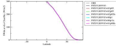
rsdscrezon
