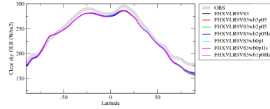
rlutcrezon
