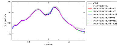
rlutzone
