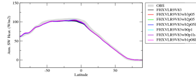
rsahzone
