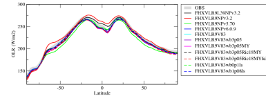
rlutzon
