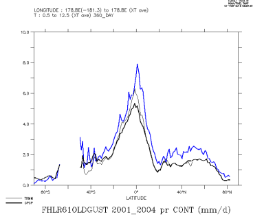
FHLR61OLDGUST_2001_2004_con
