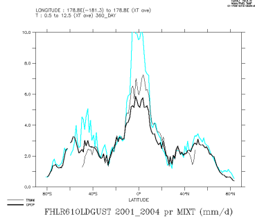
FHLR61OLDGUST_2001_2004_mix
