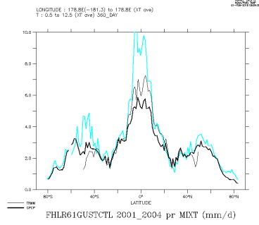
FHLR61GUSTCTL_2001_2004_mix
