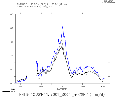
FHLR61GUSTCTL_2001_2004_con
