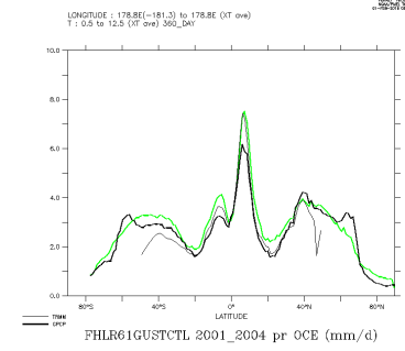
FHLR61GUSTCTL_2001_2004_oce
