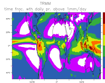
TRMM_nd
