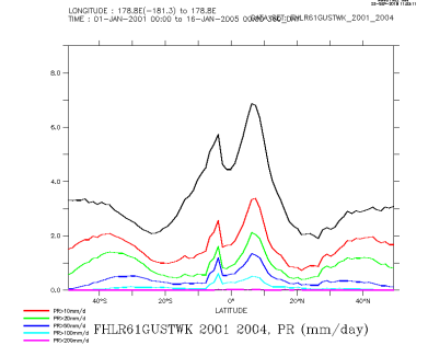
FHLR61GUSTWK_2001_2004_zon
