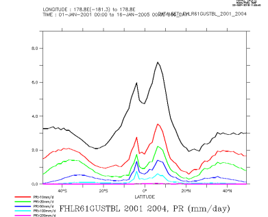
FHLR61GUSTBL_2001_2004_zon
