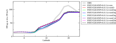
rsuscszon
