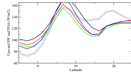
rsutazon
