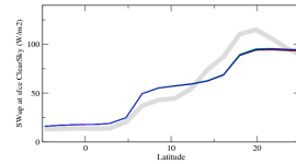
rsuscson
