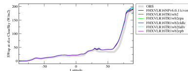
rsuscscszon
