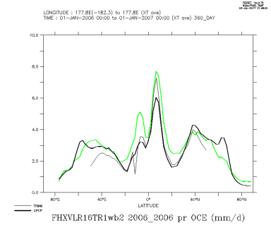
FHXVLR16TR1wb2_2006_2006_oce
