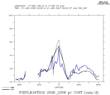
FHXVLR16TR10_2006_2006_con
