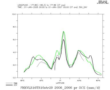
FHXVLR16TR10str20_2006_2006_oce
