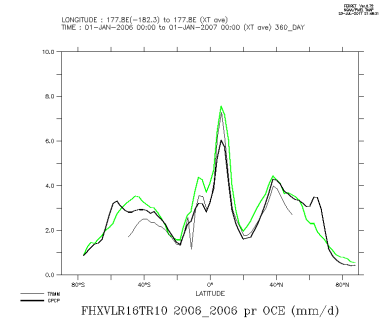
FHXVLR16TR10_2006_2006_oce
