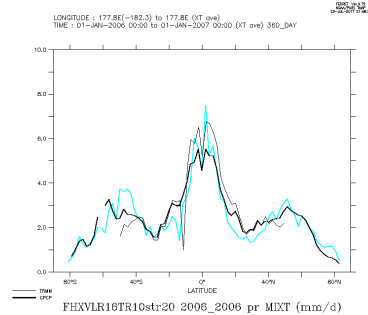
FHXVLR16TR10str20_2006_2006_mix
