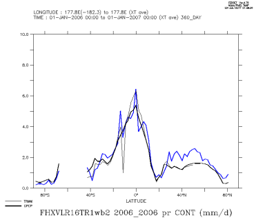
FHXVLR16TR1wb2_2006_2006_con
