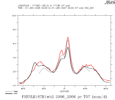
FHXVLR16TR1wb2_2006_2006_tot
