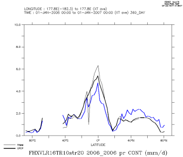
FHXVLR16TR10str20_2006_2006_con
