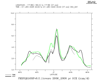
FHXVLR16NPv6.0.11cavoro_2006_2006_o
