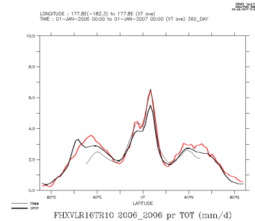
FHXVLR16TR10_2006_2006_tot
