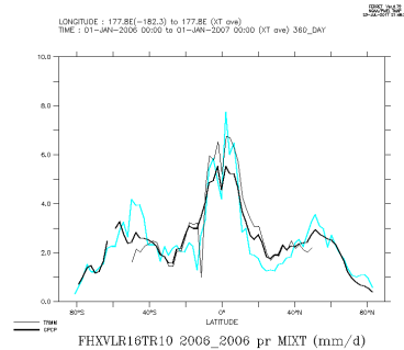
FHXVLR16TR10_2006_2006_mix
