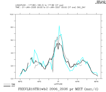
FHXVLR16TR1wb2_2006_2006_mix
