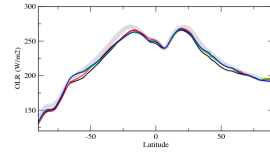
rlutzon
