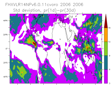
TRMM_hf
