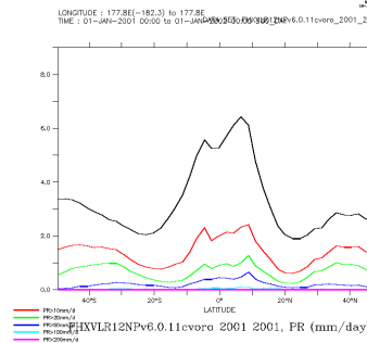
FHXVLR12NPv6.0.11cvoro_2001_2001_zon
