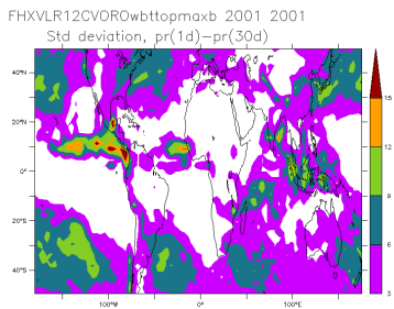
FHXVLR12NPv6.0.11cvoro_2001_2001_hf
