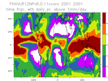
FHXVLR12NPv6.0.11gust_2001_2001_nd
