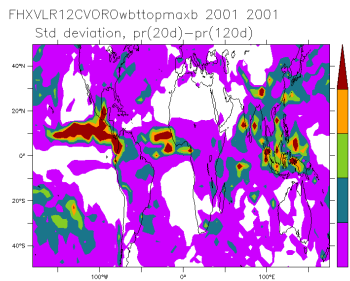
FHXVLR12NPv6.0.11cvoro_2001_2001_is
