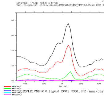
FHXVLR12NPv6.0.11gust_2001_2001_zon
