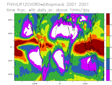
FHXVLR12NPv6.0.11cvoro_2001_2001_nd
