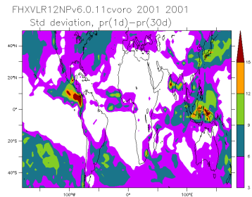
FHXVLR12NPv6.0.11gust_2001_2001_hf
