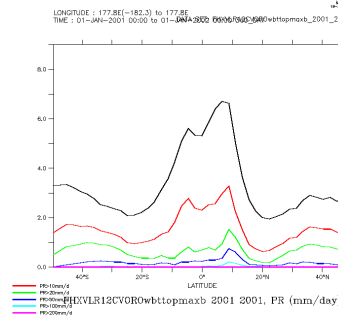
FHXVLR12CVORObttopmaxb_2001_2001_zon
