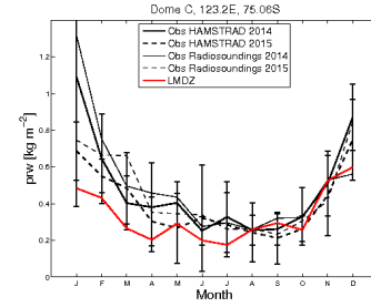
prw_DC_FHXVLR11CVOROalph07_2001_2001
