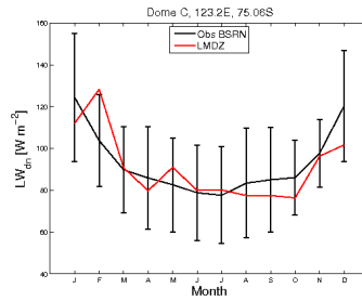
LWdnSFC_DC_FHXVLR11NPv6.0.11cvaro_2001_2001
