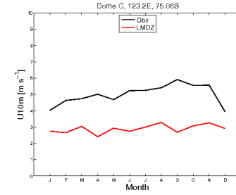
wind10m_DC_FHXVLR11CVOROalph07_2001_2001
