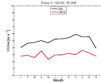
wind10m_DC_FHXVLR11CVOROt1crit45_2001_2001
