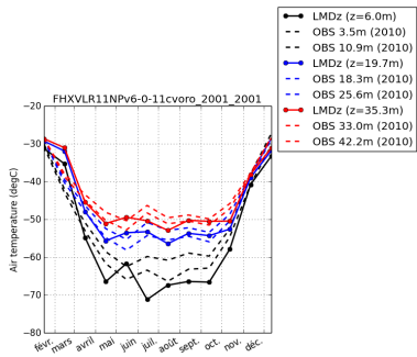
tempDC-FHXVLR11NPv6-0-11cvaro_2001_2001
