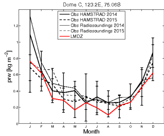
prw_DC_FHXVLR11CVOROt1crit45_2001_2001
