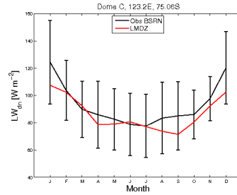
LWdnSFC_DC_FHXVLR11CVOROt1crit50_2001_2001
