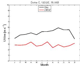
wind10m_DC_FHXVLR11CVOROalph05_2001_2001
