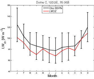
LWdnSFC_DC_FHXVLR11CVOROalph07_2001_2001
