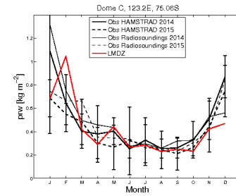
prw_DC_FHXVLR11NPv6.0.11cvaro_2001_2001
