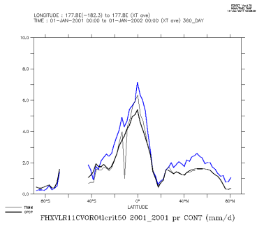
FHXVLR11CVOROtlerit50_2001_2001_con
