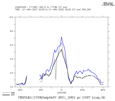
FHXVLR11CVOROalph07_2001_2001_con
