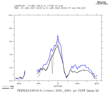
FHXVLR11NPv6.0.11cvoro_2001_2001_con
