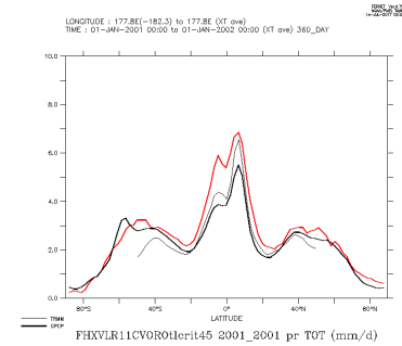
FHXVLR11CVOROtlerit45_2001_2001_tot
