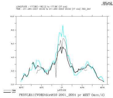
FHXVLR11CVOROtlerit50_2001_2001_mix
