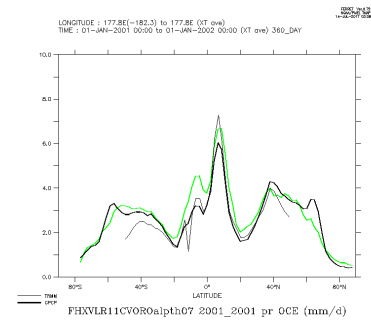
FHXVLR11CVOROalph07_2001_2001_oce
