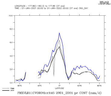
FHXVLR11CVOROtlerit45_2001_2001_con
