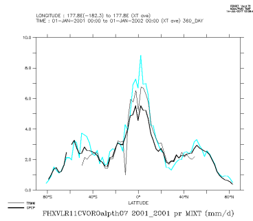
FHXVLR11CVOROalph07_2001_2001_mix
