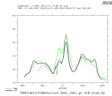
FHXVLR11CVOROtlerit45_2001_2001_oce
