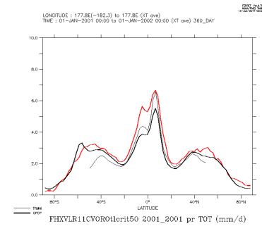
FHXVLR11CVOROtlerit50_2001_2001_tot
