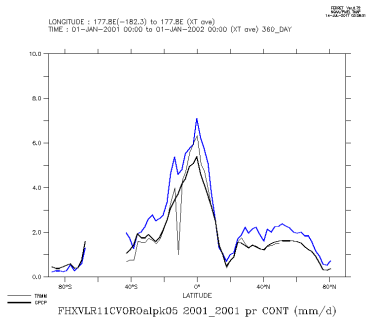
FHXVLR11CVOROalpk05_2001_2001_con
