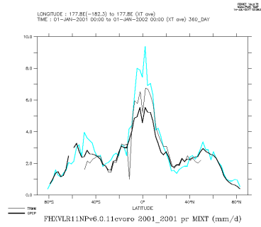
FHXVLR11NPv6.0.11cvoro_2001_2001_mix
