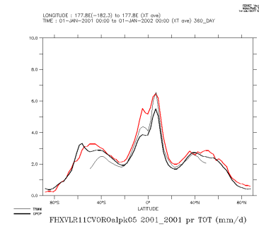
FHXVLR11CVOROalpk05_2001_2001_tot
