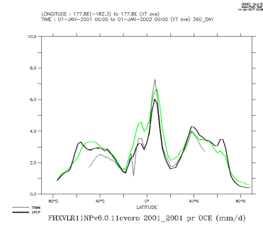
FHXVLR11NPv6.0.11cvoro_2001_2001_oce
