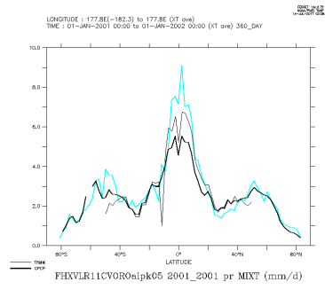
FHXVLR11CVOROalpk05_2001_2001_mix
