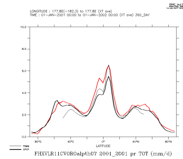
FHXVLR11CVOROalph07_2001_2001_tot
