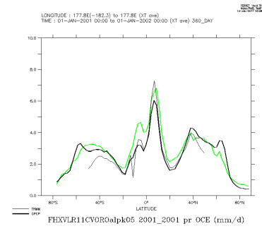
FHXVLR11CVOROalpk05_2001_2001_o
