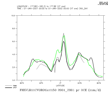
FHXVLR11CVOROtlerit50_2001_2001_oce
