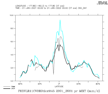
FHXVLR11CVOROtlerit45_2001_2001_mix
