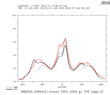
FHXVLR11NPv6.0.11cvoro_2001_2001_tot
