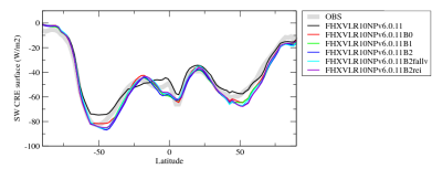
crest3zon
