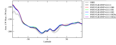
rlahzcn
