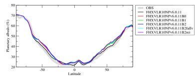
albt3zon
