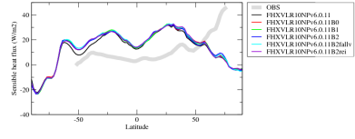
hfss3zon
