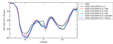
crest3zon
