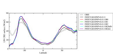
crest3zon
