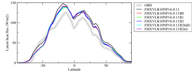
hfls3zon
