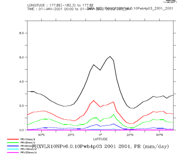
FHXVLR10NPv6.0.10Pwb4p03_2001_2001_zon
