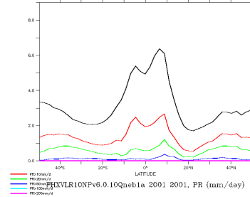
FHXVLR10NPv6.0.10Qneb1a_2001_2001_nd
