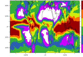
FHXVLR10NPv6.0.10Qneb1 2001 2001 time frac. with daily pr. above 1mm/day
