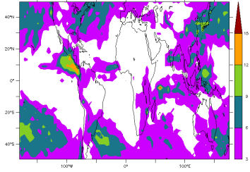
FHXVLR10NPv6.0.10Qneb1 2001 2001 Std deviation, pr(1d)-pr(30d)
