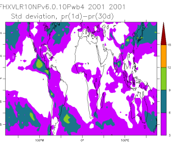
FHXVLR10NPv6.0.10P_2001_2001_hf
