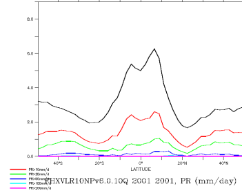
FHXVLR10NPv6.0.10Q_2001_2001_nd
