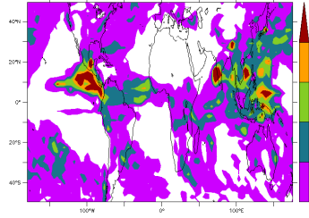
FHXVLR10NPv6.0.10Q 2001 2001 Std deviation, pr(20d)-pr(120d)
