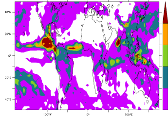
FHXVLR10NPv6.0.10Qneb1a 2001 2001 Std deviation, pr(20d)-pr(120d)
