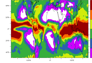
FHXVLR10NPv6.0.10Qneb0 2001 2001 time frac. with daily pr. above 1mm/day
