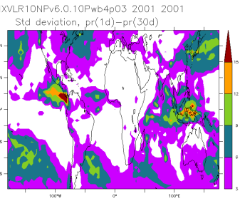
FHXVLR10NPv6.0.10Pwb4_2001_2001_hf
