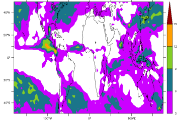
FHXVLR10NPv6.0.10Qneb1a 2001 2001 Std deviation, pr(1d)-pr(30d)
