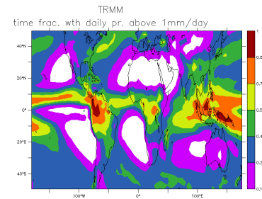
TRMM_nd
