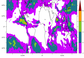
FHXVLR10NPv6.0.10Qneb0 2001 2001 Std deviation, pr(1d)-pr(30d)
