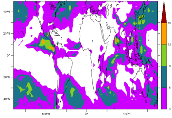
FHXVLR10NPv6.0.10Q 2001 2001 Std deviation, pr(1d)-pr(30d)
