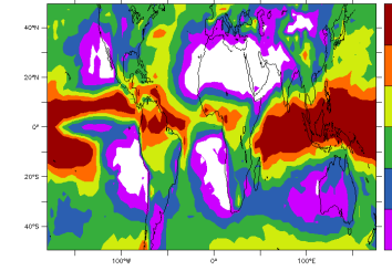
FHXVLR10NPv6.0.10Qneb1a 2001 2001 time frac. with daily pr. above 1mm/day
