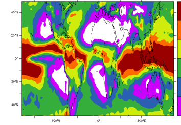
FHXVLR10NPv6.0.10Q 2001 2001 time frac. with daily pr. above 1mm/day
