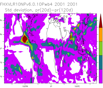
FHXVLR10NPv6.0.10P_2001_2001_is
