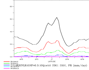
FHXVLR10NPv6.0.10Qneb0_2001_2001_nd
