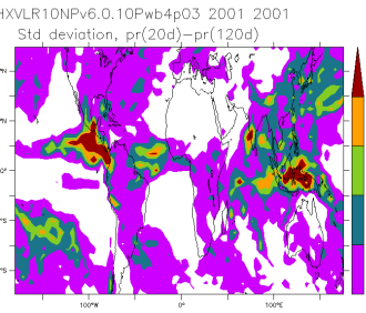
FHXVLR10NPv6.0.10Pwb4_2001_2001_is
