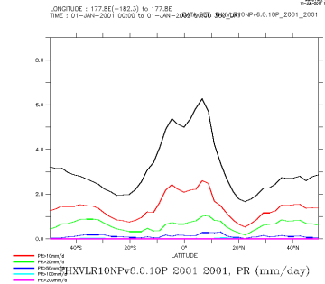
FHXVLR10NPv6.0.10P_2001_2001_zon
