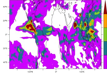
FHXVLR10NPv6.0.10Qneb0 2001 2001 Std deviation, pr(20d)-pr(120d)
