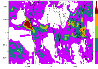
FHXVLR10NPv6.0.10Qneb1 2001 2001 Std deviation, pr(20d)-pr(120d)
