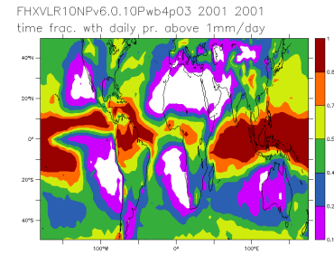
FHXVLR10NPv6.0.10Pwb4_2001_2001_nd
