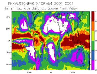
FHXVLR10NPv6.0.10P_2001_2001_nd
