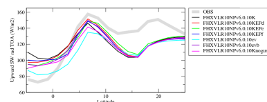
rsuscszon
