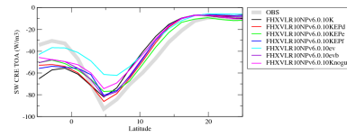
crestzon
