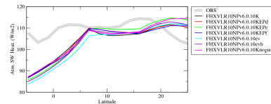
rsahzn
