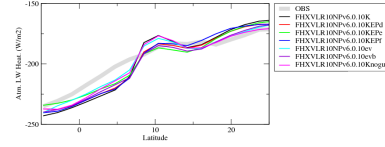
rlahzn
