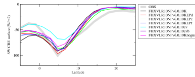
crosson
