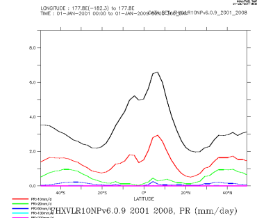
FHXVLR10NPv6.0.9_2001_2008_zon
