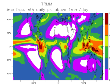
TRMM_nd
