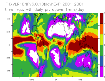
FHXVLR10NPv6.0.10blcvhEvP_2001_2001_nd
