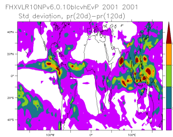
FHXVLR10NPv6.0.10blcvhEvP_2001_2001_is
