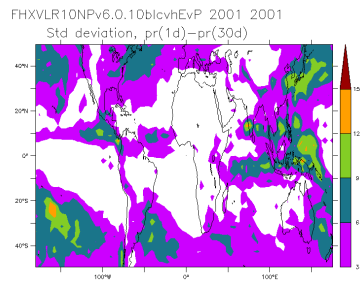
FHXVLR10NPv6.0.10blcvhEvP_2001_2001_hf
