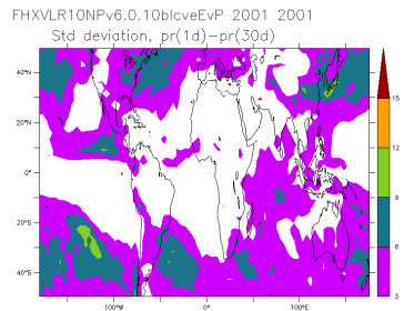
FHXVLR10NPv6.0.10blcveEvP_2001_2001_hf
