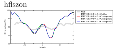
hflsazon
