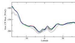
rlahzon
