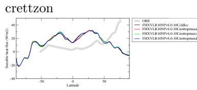
hflsazon
