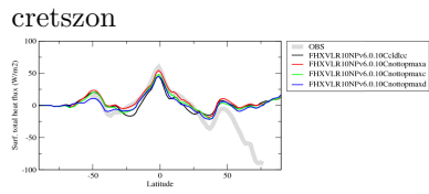
hflsazon
