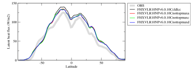
hflsazon
