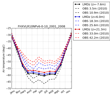
tempDC-FHXVLR10NPv6-0-10_2001_2008
