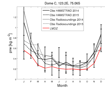
prw_DC_FHXVLR10NPv6.0.10_2001_2008
