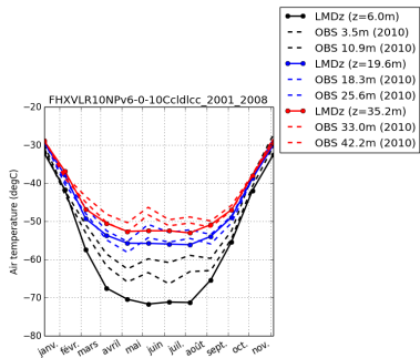
tempDC-FHXVLR10NPv6-0-10Cldlcc_2001_2008
