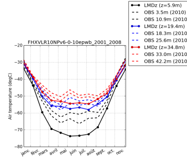
tempDC-FHXVLR10NPv6-0-10epwb_2001_2008
