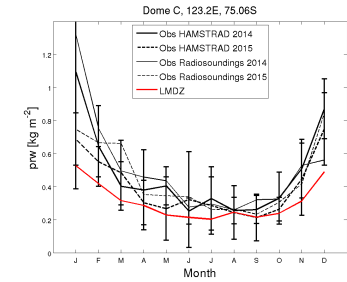
prw_DC_FHXVLR10NPv6.0.10blcv_2001_2008
