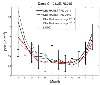
prw_DC_FHXVLR10NPv6.0.10Cldlca_2001_2008
