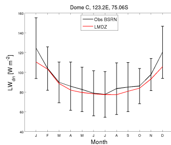
LWdnSFC_DC_FHXVLR10NPv6.0.10Cldlcc_2001_2008
