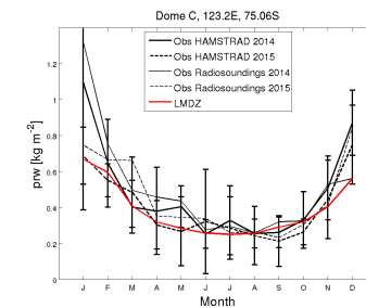
prw_DC_FHXVLR10NPv6.0.10Cldlcc_2001_2008
