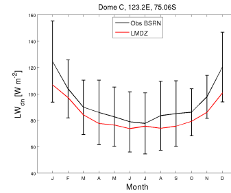
LWdnSFC_DC_FHXVLR10NPv6.0.10epwb_2001_2008
