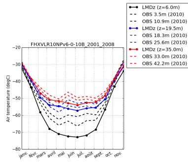
tempDC-FHXVLR10NPv6-0-10B_2001_2008
