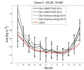
prw_DC_FHXVLR10NPv6.0.10epqrh_2001_2008
