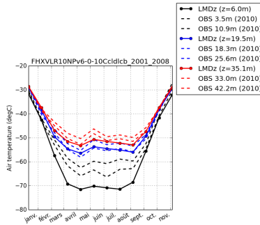
tempDC-FHXVLR10NPv6-0-10Cldlcb_2001_2008
