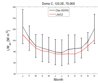
LWdnSFC_DC_FHXVLR10NPv6.0.10B_2001_2008
