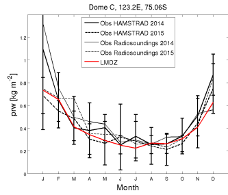
prw_DC_FHXVLR10NPv6.0.10C_2001_2008
