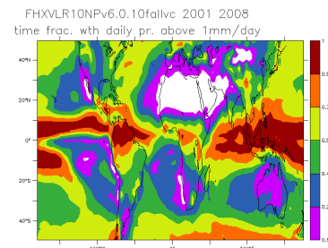
FHXVLR10NPv6.0.10_2001_2008_nd
