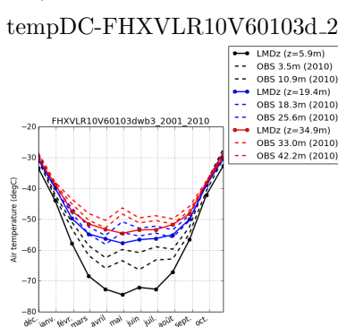
tempDC-FHXVLR10V60103dwb3_2001_2010
