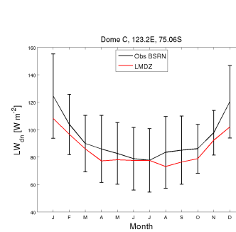
LWdnSFC_DC_FHXVLR10V60103coefeva_2001_2010
