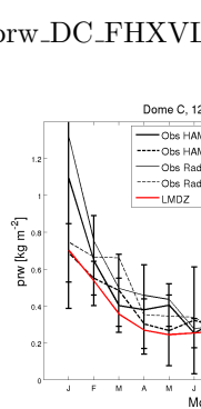
prw_DC_FHXVLR10V60103d_2001_2010
