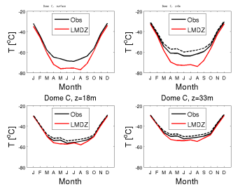
temp_DC_FHXVLR10V60103dwb3p02_2001_2010
