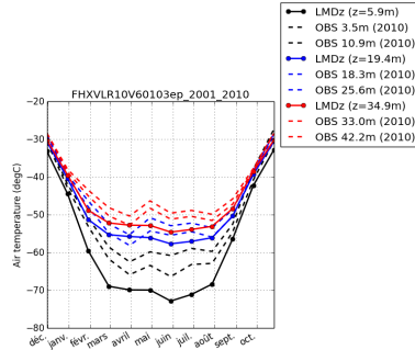
tempDC-FHXVLR10V60103ep_2001_2010
