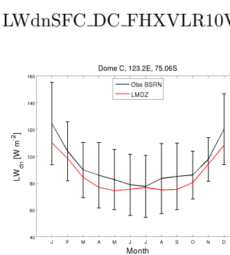
LWdnSFC_DC_FHXVLR10V60103d_2001_2010
