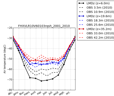
tempDC-FHXVLR10V60103rqsh_2001_2010
