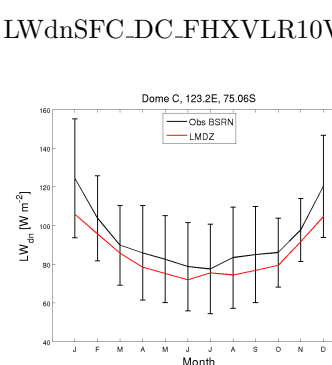
LWdnSFC_DC_FHXVLR10V60103dwb3_2001_2010
