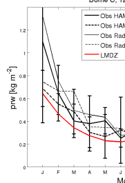
prw_DC_FHXVLR10V60103epgust_2001_2010
