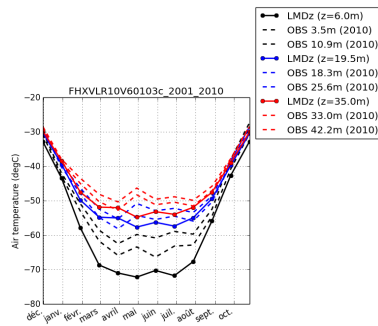
tempDC-FHXVLR10V60103c_2001_2010
