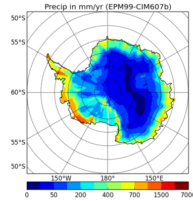
precipSH-EPM99-CIM607b
