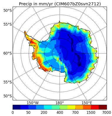
precipSH-CIM607bZ0svn2712
