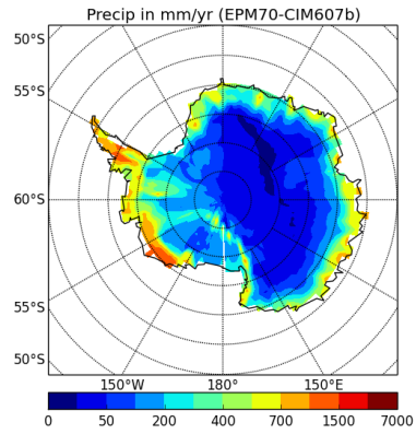
precipSH-EPM70-CIM607b
