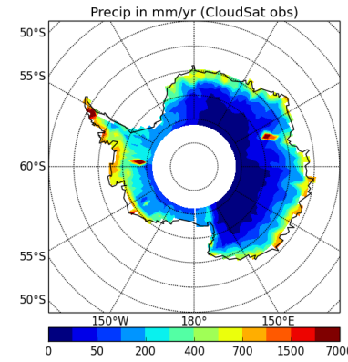
precipSH-OBS
