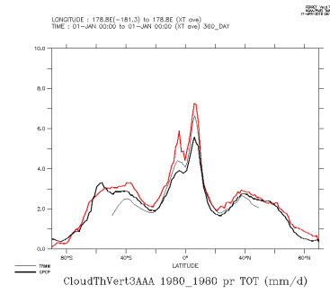
CloudThVert3AAA_1980_1980_tot
