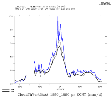
CloudThVert3AAA_1980_1980_con
