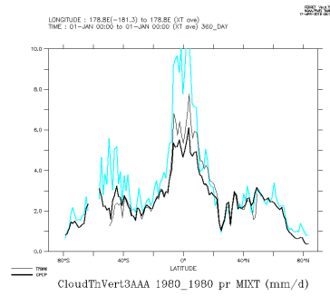
CloudThVert3AAA_1980_1980_mix
