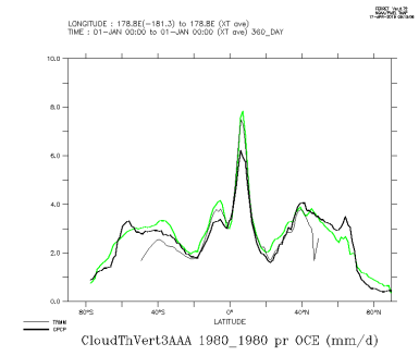
CloudThVert3AAA_1980_1980_oce
