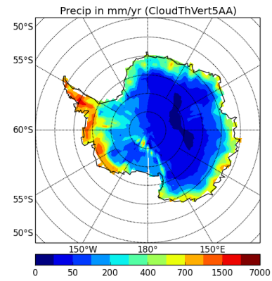
precipSH-CloudThVert5AA
