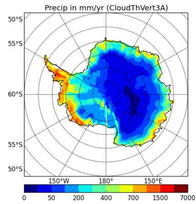
precipSH-CloudThVert3A
