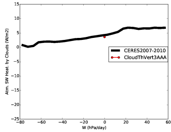
rsahcre_CldThT0
