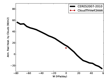
rahcre_CldThT0
