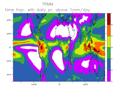
TRMM_nd
