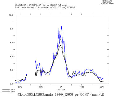
CL4.4365.L2883.usda.1999_2008_con
