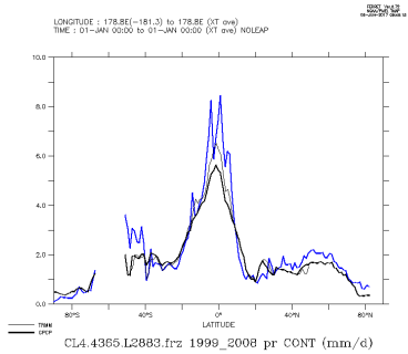
CL4.4365.L2883.frz.1999_2008_con
