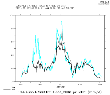
CL4.4365.L2883.frz.1999_2008_mix
