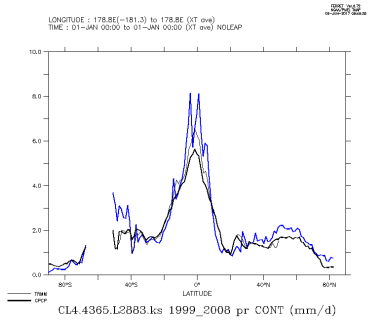
CL4.4365.L2883.ks.1999_2008_con
