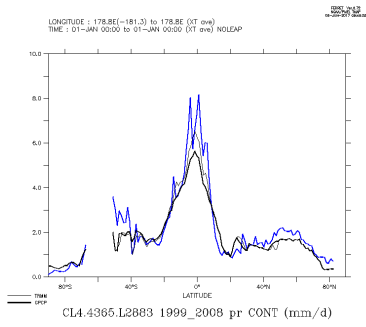
CL4.4365.L2883_1999_2008_con
