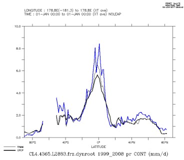
CL4.4365.L2883.frz.dynroot.1999_2008_con
