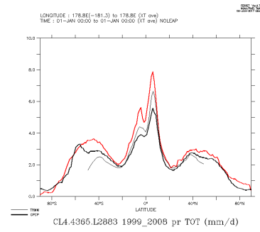
CL4.4365.L2883_1999_2008_tot
