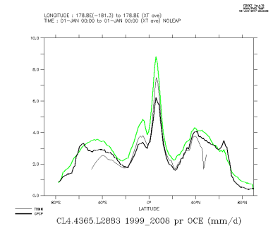
CL4.4365.L2883_1999_2008_oce
