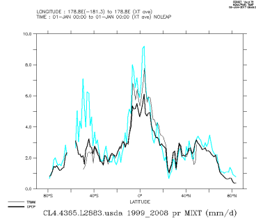
CL4.4365.L2883.usda.1999_2008_mix
