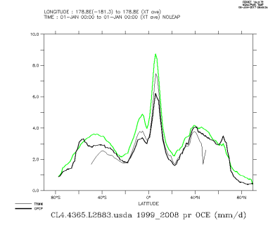
CL4.4365.L2883.usda.1999_2008_oce
