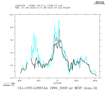
CL4.4365.L2883.ks.1999_2008_mix
