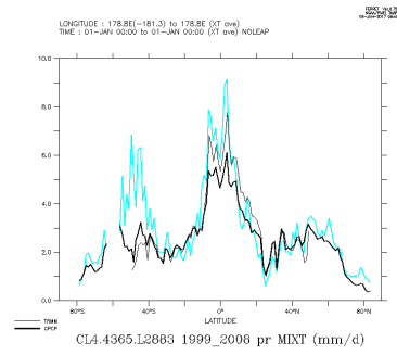
CL4.4365.L2883_1999_2008_mix
