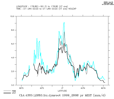
CL4.4365.L2883.frz.dynroot.1999_2008_mix
