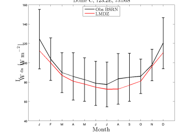
LWdn_DC.NSTOZ0SNOWroot_1980_1989
