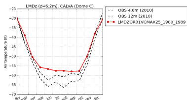
tempDC-LMDZOR01VCMAX25_1980_1989
