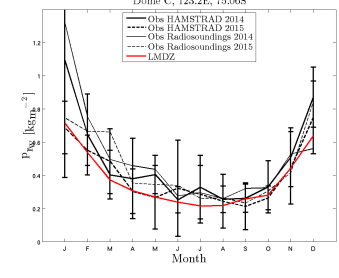
prw_DC.NSTOZ0SNOWroot_1980_1989
