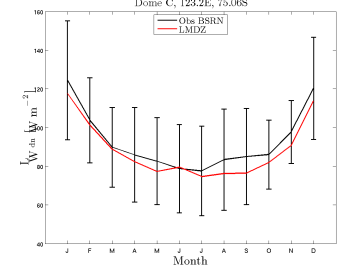
LWdn_DC.LMDZOR01_1980_1989
