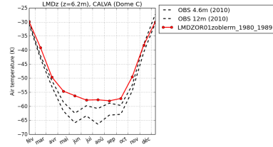
tempDC-LMDZOR01zoblerm_1980_1989
