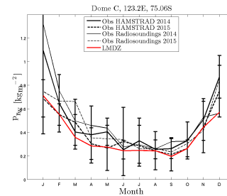
prw_DC LMDZOR01VCMAX25_1980_1989
