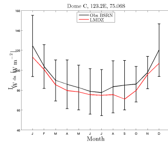
LWdn_DC LMDZOR01VCMAX25_1980_1989
