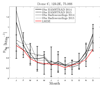
prw_DC NSTOZ0SNOWO2_1980_1989
