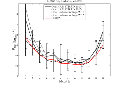
prw_DC.NSTOZ0SNOW_1980_1989
