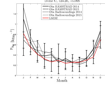
prw_DC.LMDZOR01_1980_1989
