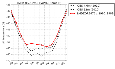
tempDC-LMDZOR3476b_1980_1989
