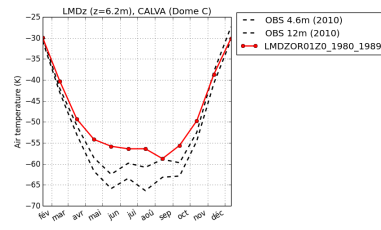
tempDC-LMDZOR01Z0_1980_1989
