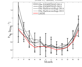
prw_DC.LMDZOR3476b_1980_1989
