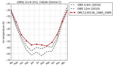
tempDC-ORC113013b_1980_1989
