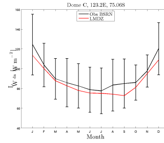
LWdn_DC LMDZOR01zoblerm_1980_1989
