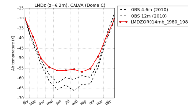
tempDC-LMDZOR014mb_1980_1989
