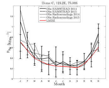
prw_DC LMDZOR01zoblerm_1980_1989
