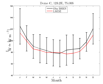
LWdn_DC LMDZOR014mb_1980_1989
