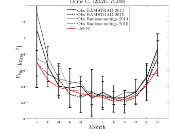
prw_DC.LMDZOR01Z0_1980_1989
