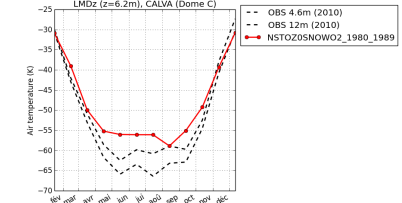
tempDC-NSTOZ0SNOWO2_1980_1989
