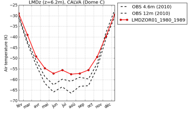
tempDC-LMDZOR01_1980_1989
