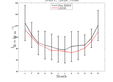
LWdn_DC.ORC113013b_1980_1989
