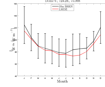
LWdn_DC.NSTOZ0SNOW_1980_1989
