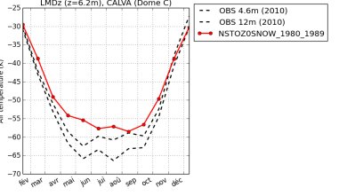
tempDC-NSTOZ0SNOW_1980_1989
