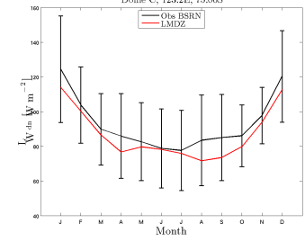
LWdn_DC.LMDZOR3476b_1980_1989
