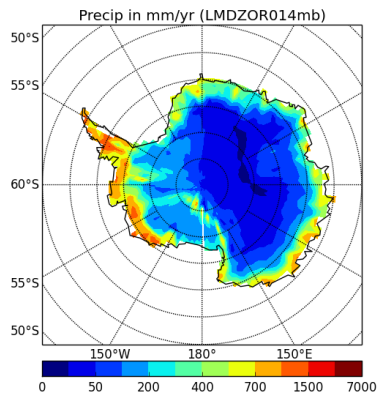
precipSH-LMDZOR14mb
