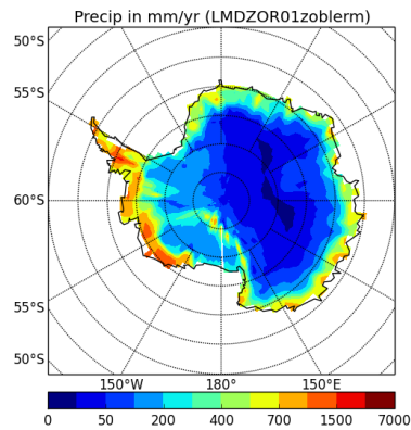
precipSH-LMDZOR1zoblrm
