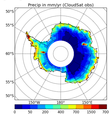
precipSH-OBS
