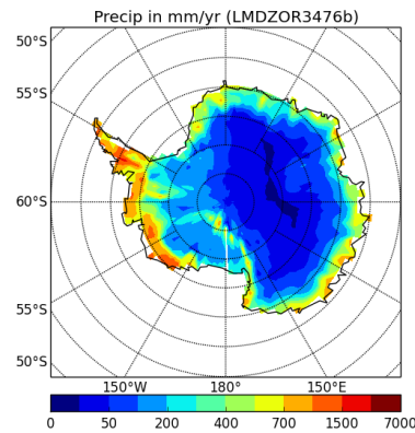
precipSH-LMDZOR3476b
