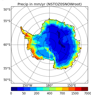
precipSH-NSTOZ0SNOWroot
