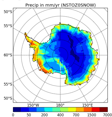
precipSH-NSTOZ0SNOW
