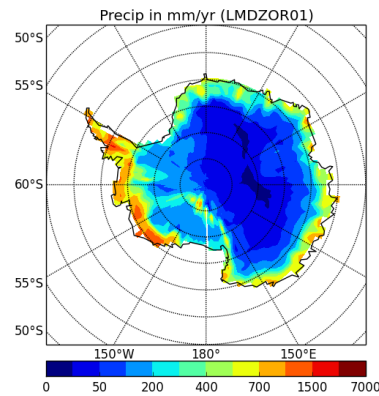
precipSH-LMDZOR1
