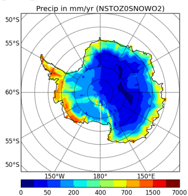
precipSH-NSTOZ0SNOW02
