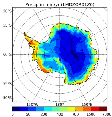
precipSH-LMDZOR1Z0
