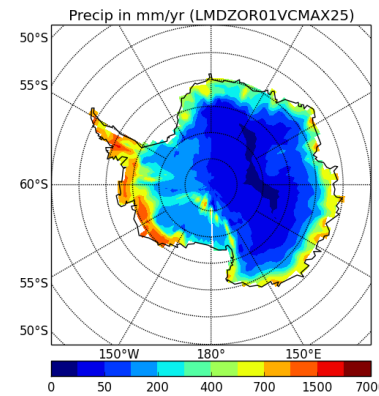
precipSH-LMDZOR1VCMAX25
