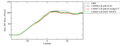
rsahzone
