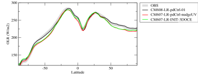
rlutzone
