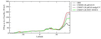
rsuscszone
