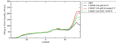
rsutcszone
