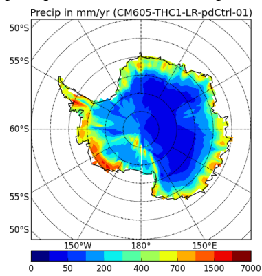
precipSH-CM605-THC1-LR-pdCtrl-01
