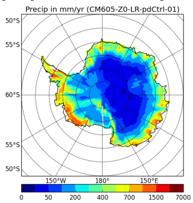
precipSH-CM605-Z0-LR-pdCtrl-01
