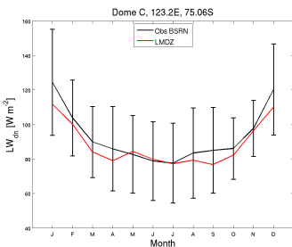
LWdnSFC_DC_CM6015-LR-amip-ttop-02_1999_2008
