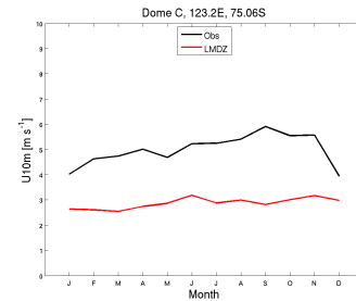
wind10m_DC_CM6015-LR-amip-split-G-02_1999_2008
