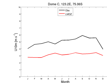
wind10m_DC_CM6015-LR-amip-ttop-02_1999_2008
