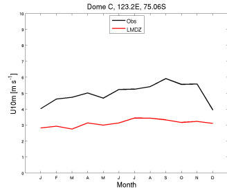
wind10m_DC_CM6015-LR-amip-split-02_1999_2008
