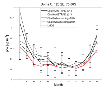
prw_DC_CM6015-LR-amip-ttop-02_1999_2008
