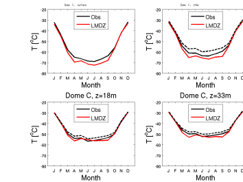
temp_DC_CM6015-LR-amip-ttop-02_1999_2008
