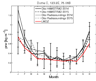
prw_DC_LMDZOR6.0.12split.Z0.NUD_2000_2009
