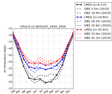
tempDC-CPL6-0-12-NOGUST_1950_1959
