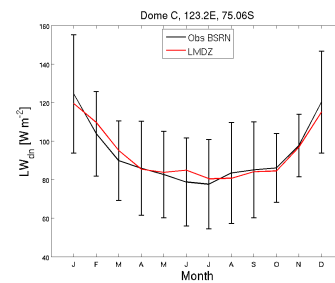
LWdnSFC_DC_CPL6.0.12.NOGUST_1950_1959
