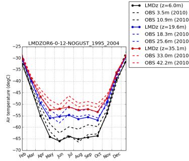
tempDC-LMDZOR6-0-12-NOGUST_1995_2004
