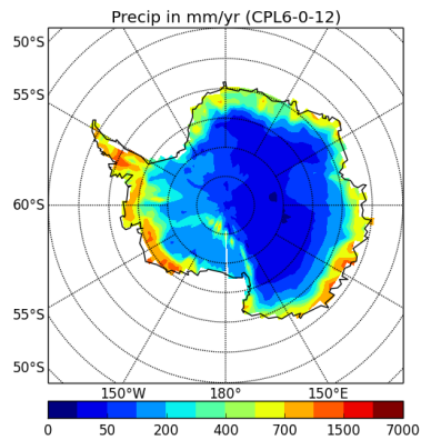
precipSH-CPL6-0-12
