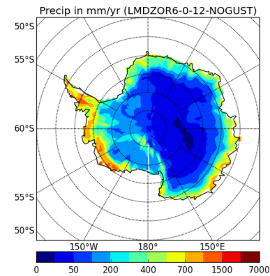
precipSH-LMDZOR6-0-12-NOGUST
