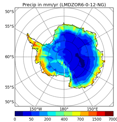
precipSH-LMDZOR6-0-12-NG
