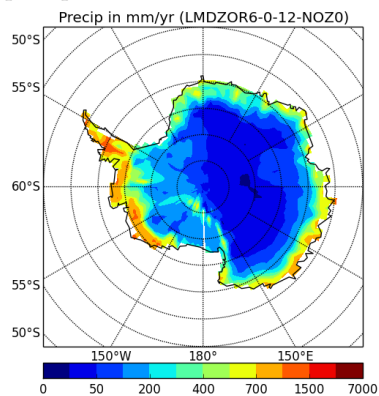
precipSH-LMDZOR6-0-12-NOZ0
