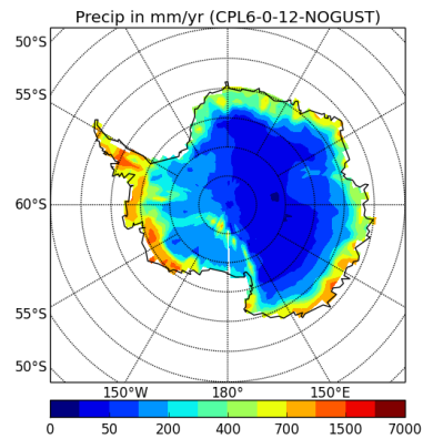
precipSH-CPL6-0-12-NOGUST
