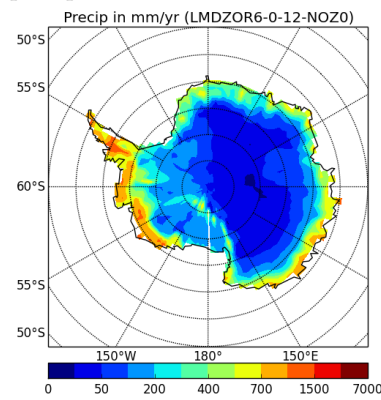
precipSH-LMDZOR6-0-12-NOZ0
