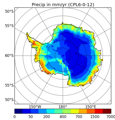
precipSH-CPL6-0-12
