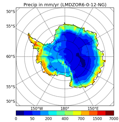
precipSH-LMDZOR6-0-12-NG
