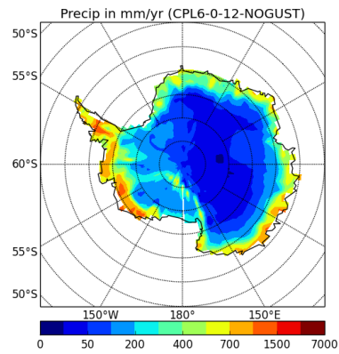
precipSH-CPL6-0-12-NOGUST
