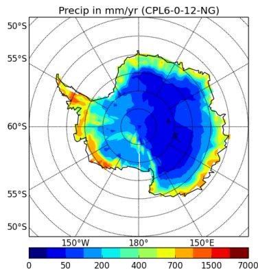
precipSH-CPL6-0-12-NG
