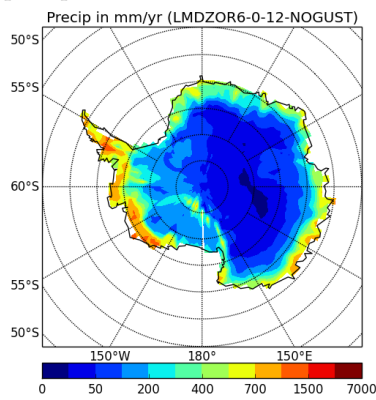
precipSH-LMDZOR6-0-12-NOGUST
