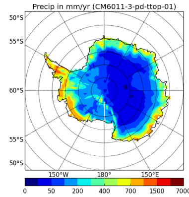
precipSH-CM6011-3-pd-ttop-01
