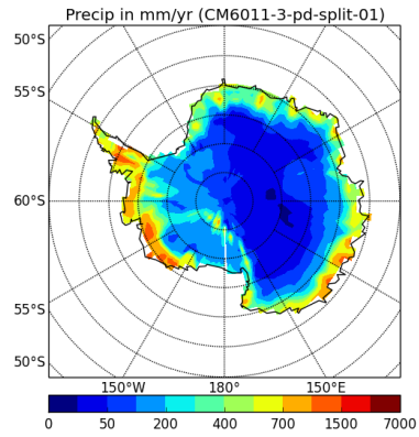
precipSH-CM6011-3-pd-split-01
