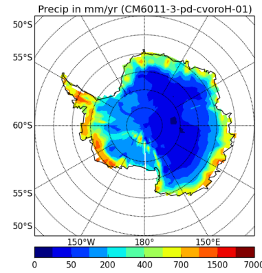
precipSH-CM6011-3-pd-cvoroH-01
