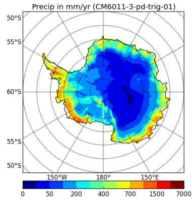
precipSH-CM6011-3-pd-trig-01
