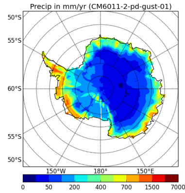
precipSH-CM6011-2-pd-gust-01
