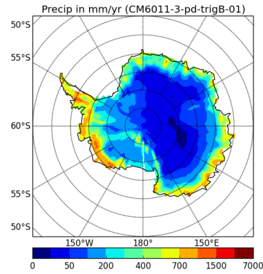
precipSH-CM6011-3-pd-trigB-01
