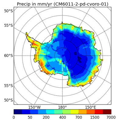
precipSH-CM6011-2-pd-cvoro-01
