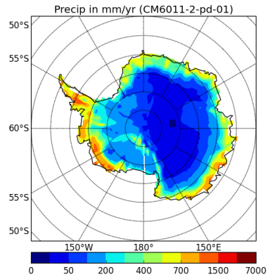
precipSH-CM6011-2-pd-01
