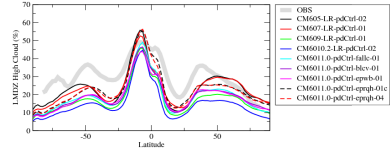
rldscrezon
