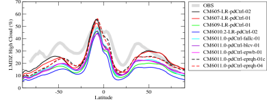
rsdscrezon
