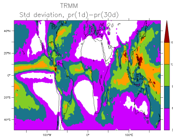
TRMM_hf
