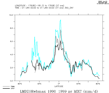
LMDZORwbmax_1990_1999_mix
