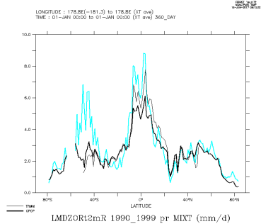
LMDZORt2mR_1990_1999_mix
