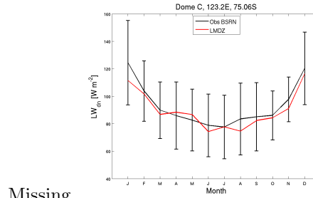
tsol_DC_REFT2M_1980.1984
