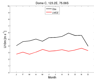
wind10m_DC_REFT2M_1980.1984
