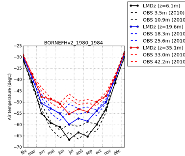
tempDC-BORNEFHv2_1980.1984
