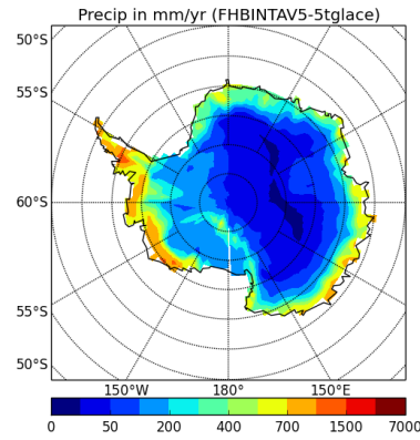
precipSH-FHBINTAV5-5tglace
