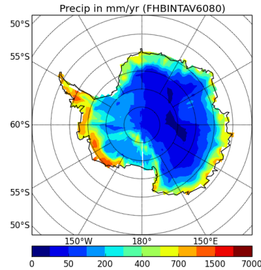
precipSH-FHBINTAV6080
