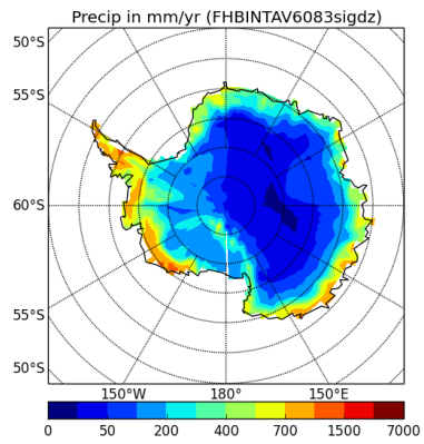
precipSH-FHBINTAV6083sigdz
