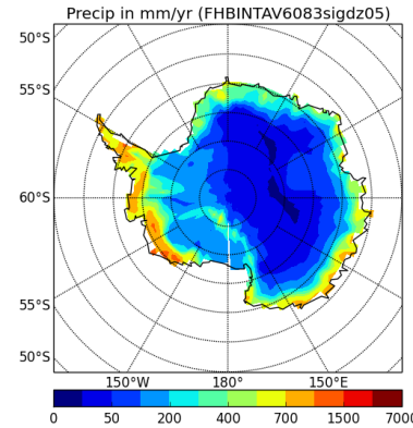
precipSH-FHBINTAV6083sigdz05
