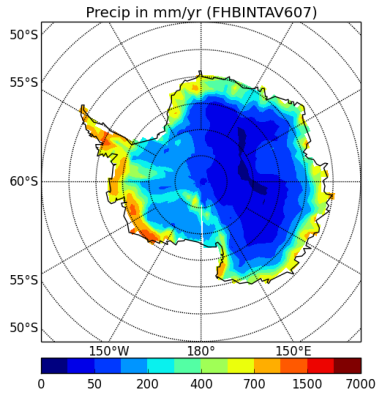
precipSH-FHBINTAV607
