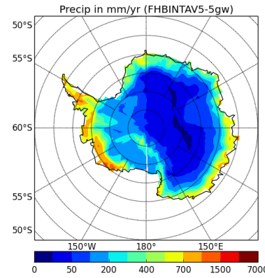
precipSH-FHBINTAV5-5gw
