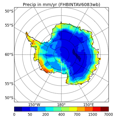
precipSH-FHBINTAV6083wb
