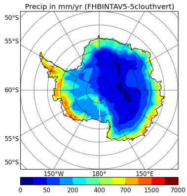
precipSH-FHBINTAV5-5clouthvert
