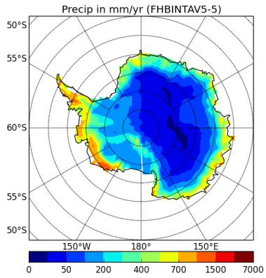
precipSH-FHBINTAV5-5
