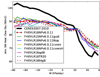
rsahcs_BEST5
