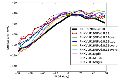
cress_BEST5
