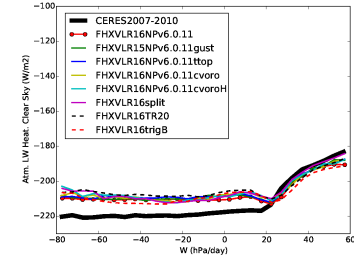
rlahcs_BEST5
