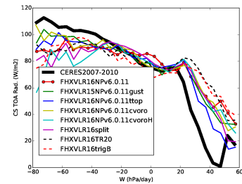
rttcs_BEST5
