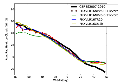
rahcre_BEST1
