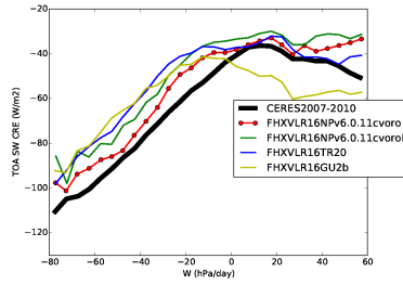
crest_BEST1
