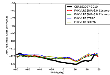
rahcs_BEST1
