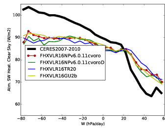
rsahcs_BEST1
