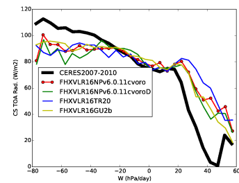
rttcs_BEST1
