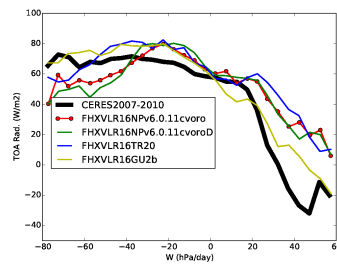
rtt_BEST1
