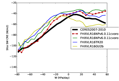
cress_BEST1
