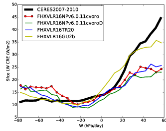
crels_BEST1
