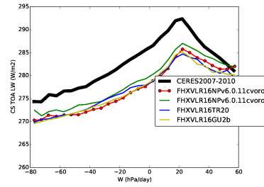
rlutcs_BEST1
