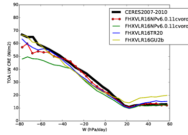
cretl_BEST1
