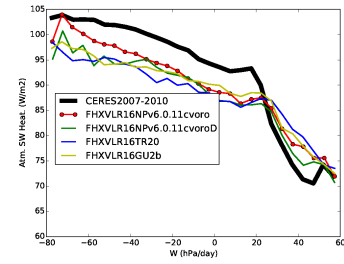
rsah_BEST1
