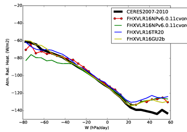
rah_BEST1
