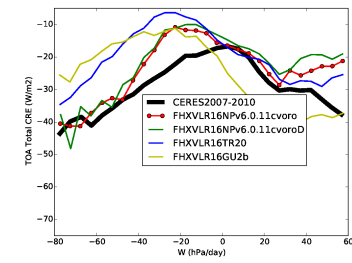
crettt_BEST1
