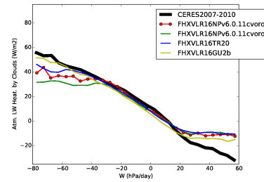
ralahcre_BEST1
