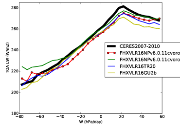
rlut_BEST1
