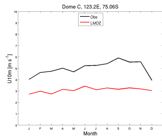
wind10m_DC_CM61-LR-amip-hist-1875-irene_1870_1879
