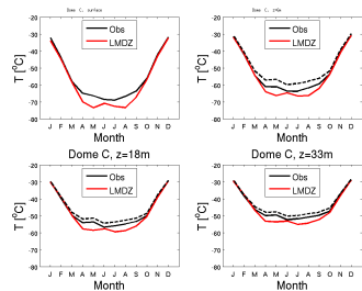
temp_DC_CM61-LR-amip-hist-1870-irene_1870_1879
