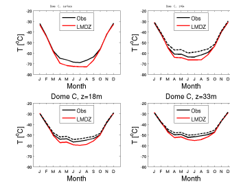
temp_DC_CM61-LR-amip-hist-1877-irene.1870-1879
