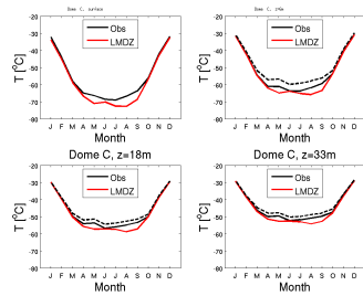
temp_DC_CM61-LR-amip-hist-1875-irene_1870_1879
