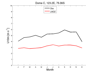
wind10m_DC_CM61-LR-amip-hist-1877-irene.1870-1879
