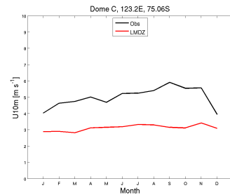
wind10m_DC_CM61-LR-amip-hist-1871-irene_1870_1879
