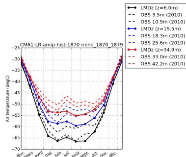
tempDC_CM61-LR-amip-hist-1870-irene_1870_1879
