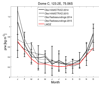
prw_DC_CM61-LR-amip-hist-1877-irene.1870-1879
