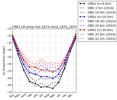
tempDC_CM61-LR-amip-hist-1874-irene_1870_1879
