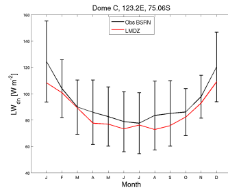
Missing tsol_DC_CM61-LR-amip-hist-1879-irene.1870-1879
