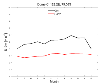
wind10m_DC_CM61-LR-amip-hist-1870-irene_1870_1879
