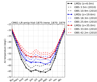
tempDC_CM61-LR-amip-hist-1875-irene_1870_1879
