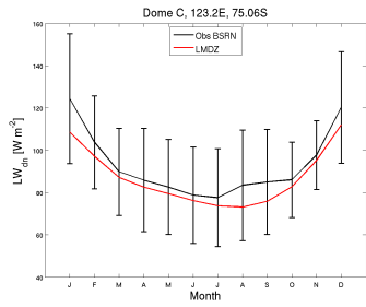
Missing tsol_DC_CM61-LR-amip-hist-1873-irene_1870_1879
