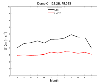
wind10m_DC_CM61-LR-amip-hist-1876-irene.1870-1879
