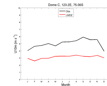
wind10m_DC_CM61-LR-amip-hist-1872-irene_1870_1879
