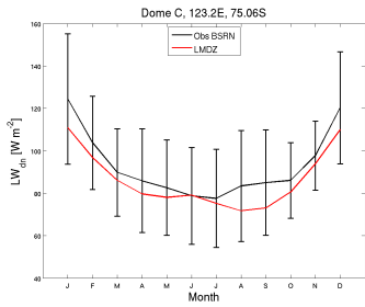
Missing tsol_DC_CM61-LR-amip-hist-1878-irene.1870-1879
