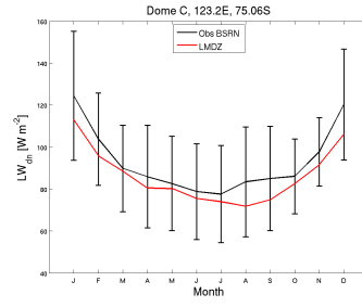
Missing tsol_DC_CM61-LR-amip-hist-1874-irene_1870_1879
