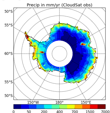
precipSH-OBS
