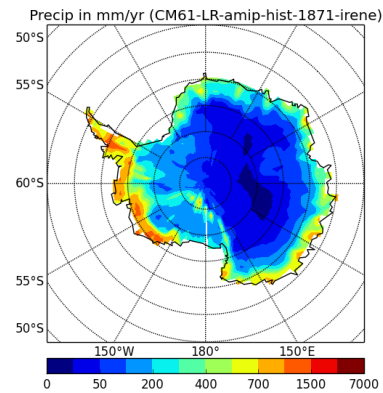
precipSH-CM61-LR-amip-hist-1871-irene
