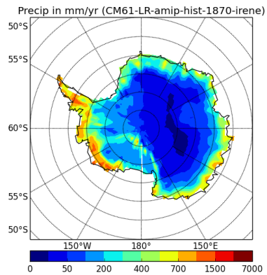
precipSH-CM61-LR-amip-hist-1870-irene
