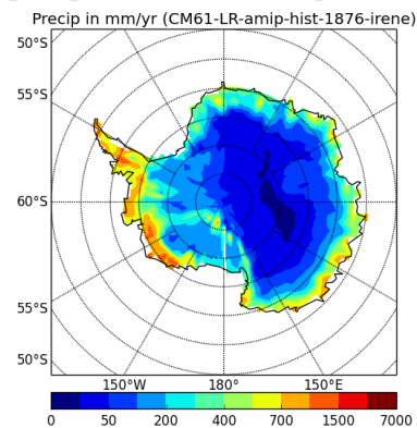
precipSH-CM61-LR-amip-hist-1876-irene
