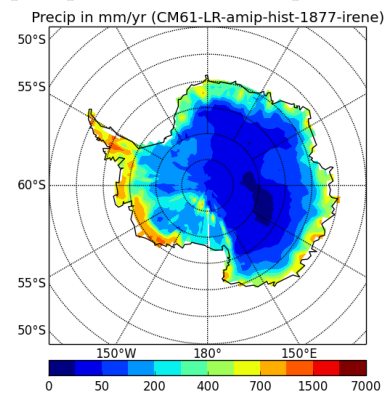
precipSH-CM61-LR-amip-hist-1877-irene
