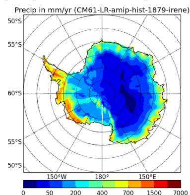
precipSH-CM61-LR-amip-hist-1879-irene
