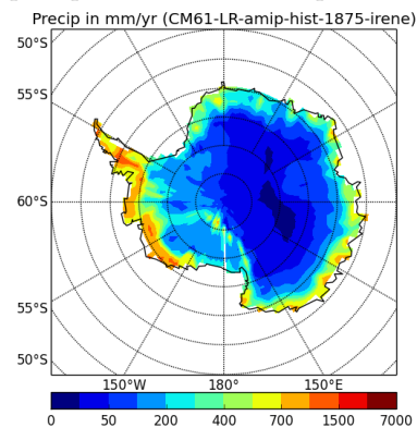
precipSH-CM61-LR-amip-hist-1875-irene
