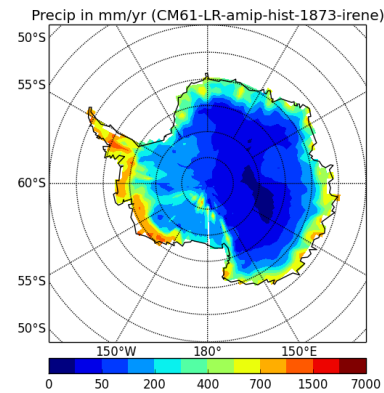
precipSH-CM61-LR-amip-hist-1873-irene
