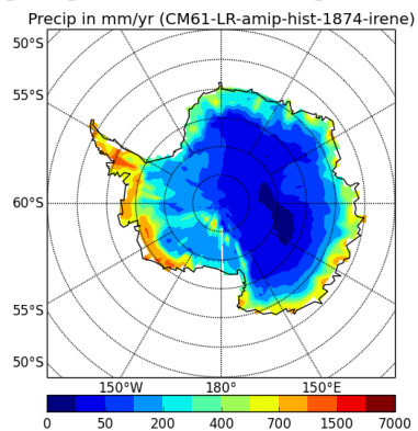
precipSH-CM61-LR-amip-hist-1874-irene
