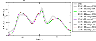
cretlson
