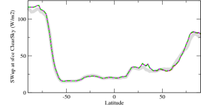
rsuscso
