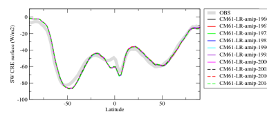
crosson
