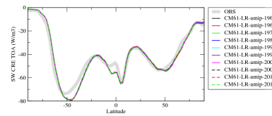
crestson
