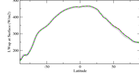
rlusczo
