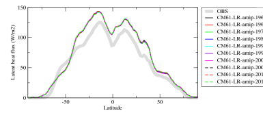
hflsazon
