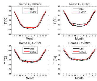
temp_DC_CM615-LR-amip-p4K-lwoff-00_2005_2014
