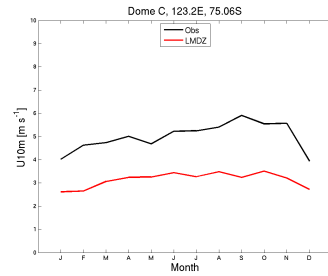
wind10m_DC_CM615-LR-amip-p4K-lwoff-00_2005_2014
