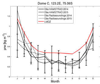
prw_DC_CM615-LR-amip-p4K-lwoff-00_2005_2014
