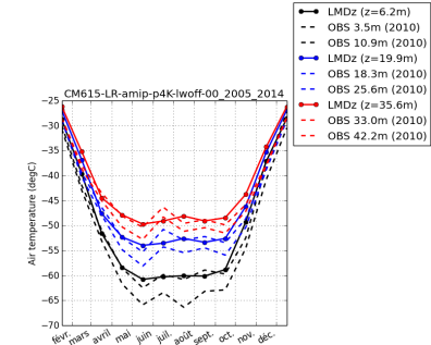
tempDC_CM615-LR-amip-p4K-lwoff-00_2005_2014
