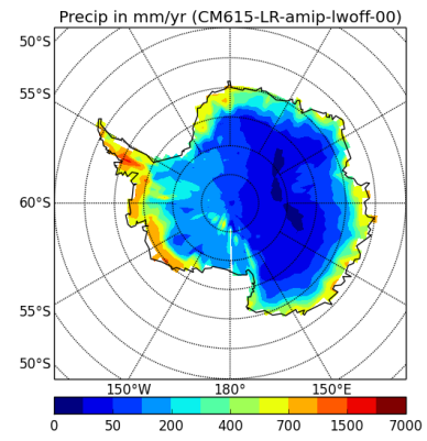
precipSH-CM615-LR-amip-lwoff-00
